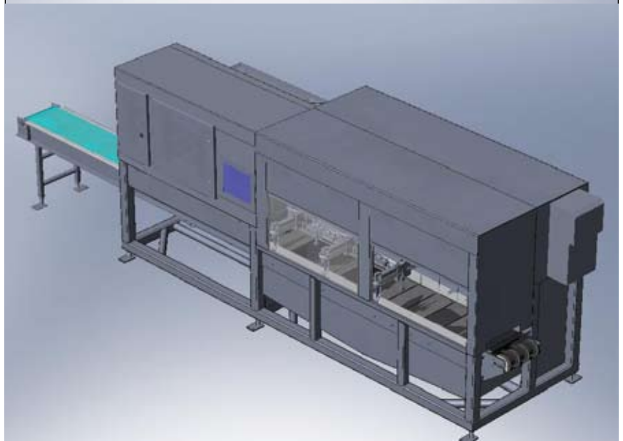
MP IntelliJet™ Water Cutter Infeed and Outfeed Views
